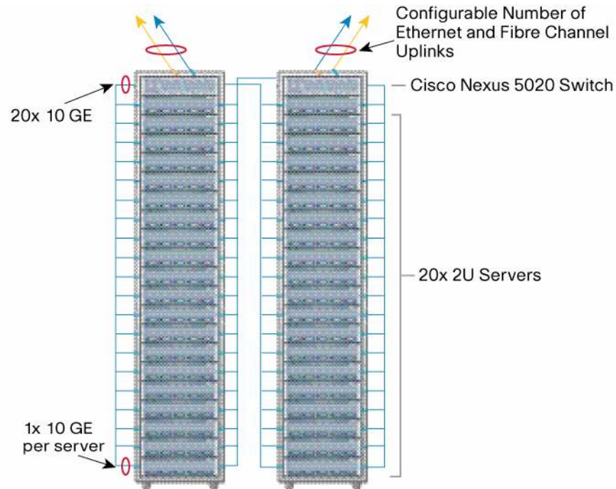
Figure 3. I/O Consolidation Scenario with Two 42RU Racks of 20 2RU Servers Each
