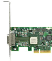
MHES14-XTC – 10Gb/s InfiniBand w/ PCI Express x4
