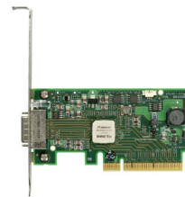
MHES18-XTC – 10Gb/s and 20Gb/s InfiniBand w/ PCI Express x4 and x8
